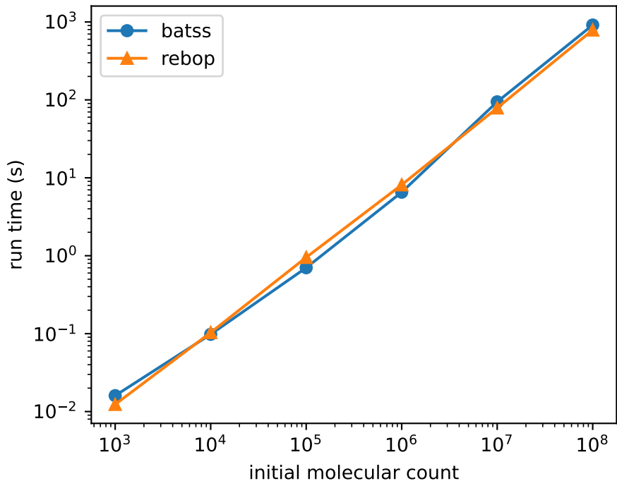
Order-3 Brusselator: run time to simulate t=40.0
